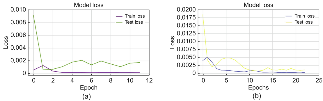
Fig. 2. Loss values of two LSTM models. (a) Loss of LSTM model. (b) Loss of Sentiment embedding LSTM model.
