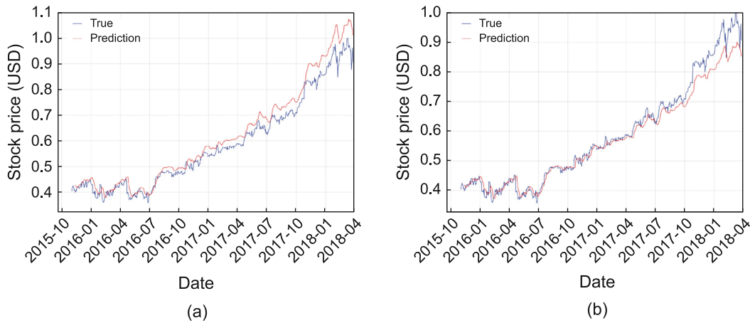
Fig. 3. Prediction results of two LSTM models. (a) Prediction results of LSTM model. (b) Prediction results of sentiment embedding LSTM model.
