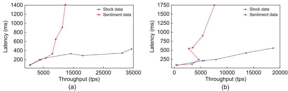
Fig. 4. Latency vs. Throughput. (a) The case of f = 1 . (b) The case of f = 5 .
